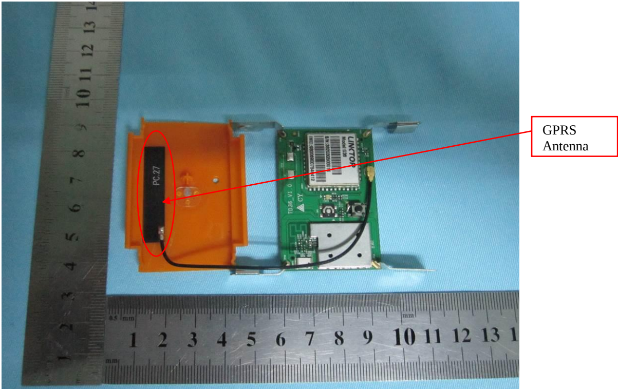
Cover Off – Main Borad View
