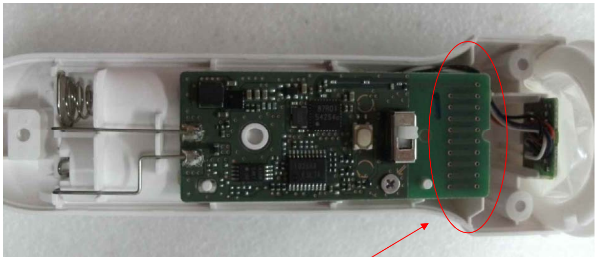
Receiving Antenna
