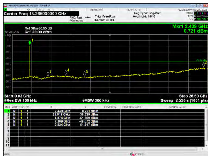
Tx. Spurious NVHT n20 2462MHz Ant1 Ref
