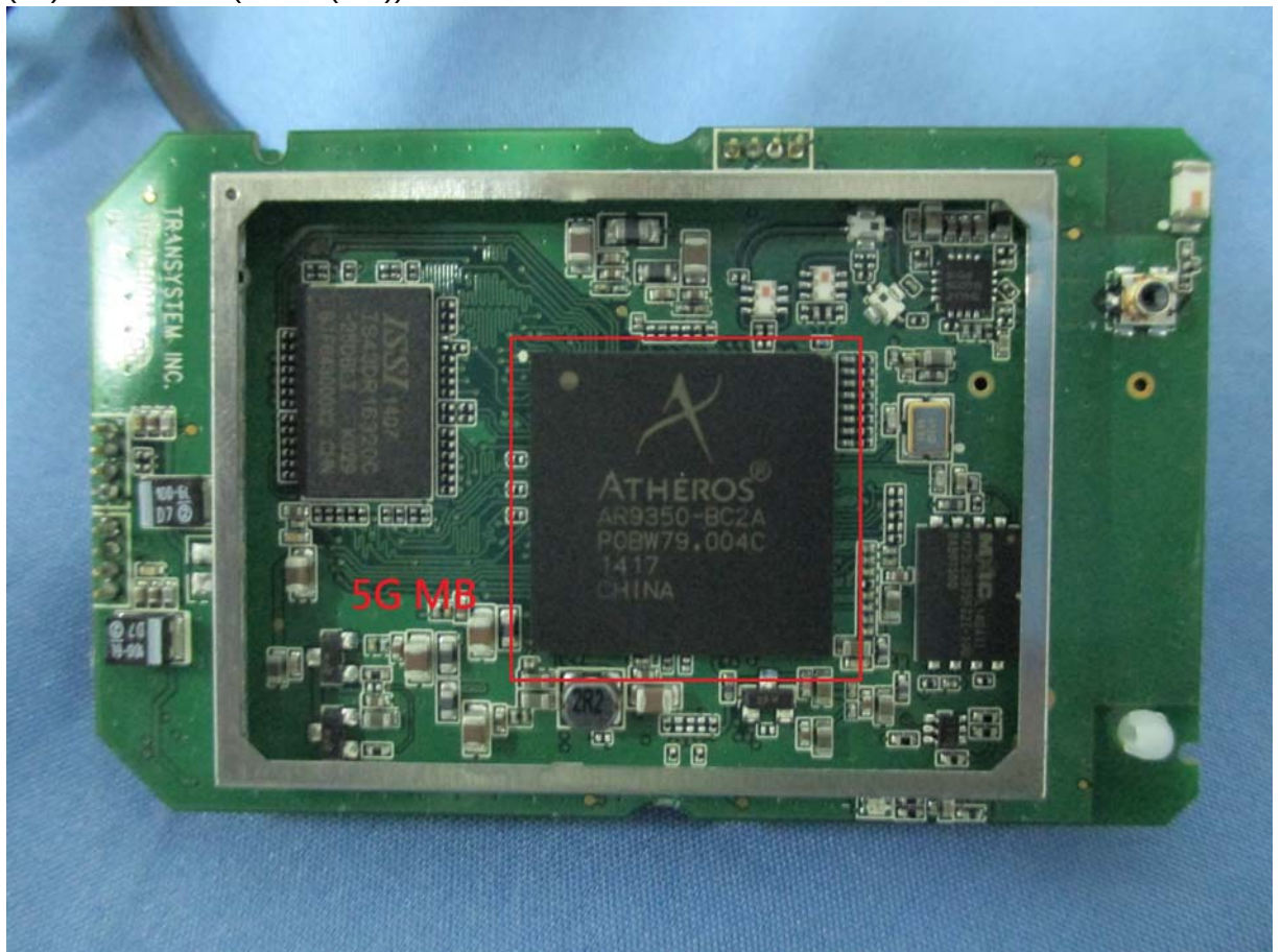
(15) EUT Photo (5GHz (MB))
