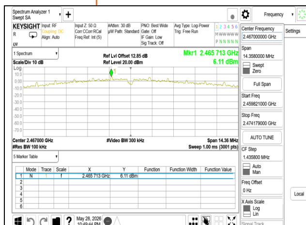
802.11g_20MHz_Chain1_2467MHz
