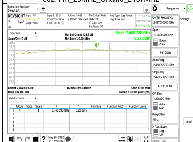
802.11n_20MHz_Chain1_2467MHz
