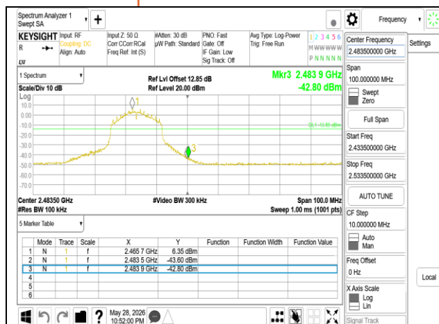
802.11g_20MHz_Chain1_2467MHz
