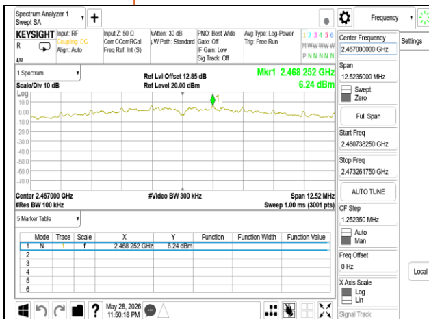
802.11ax 20MHz Chain1 2467MHz
