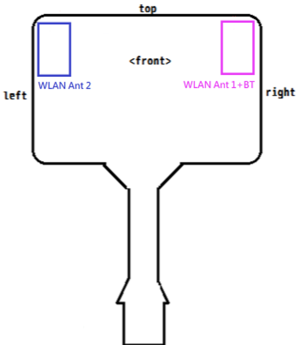
Photograph 17. Antenna position of EUT
