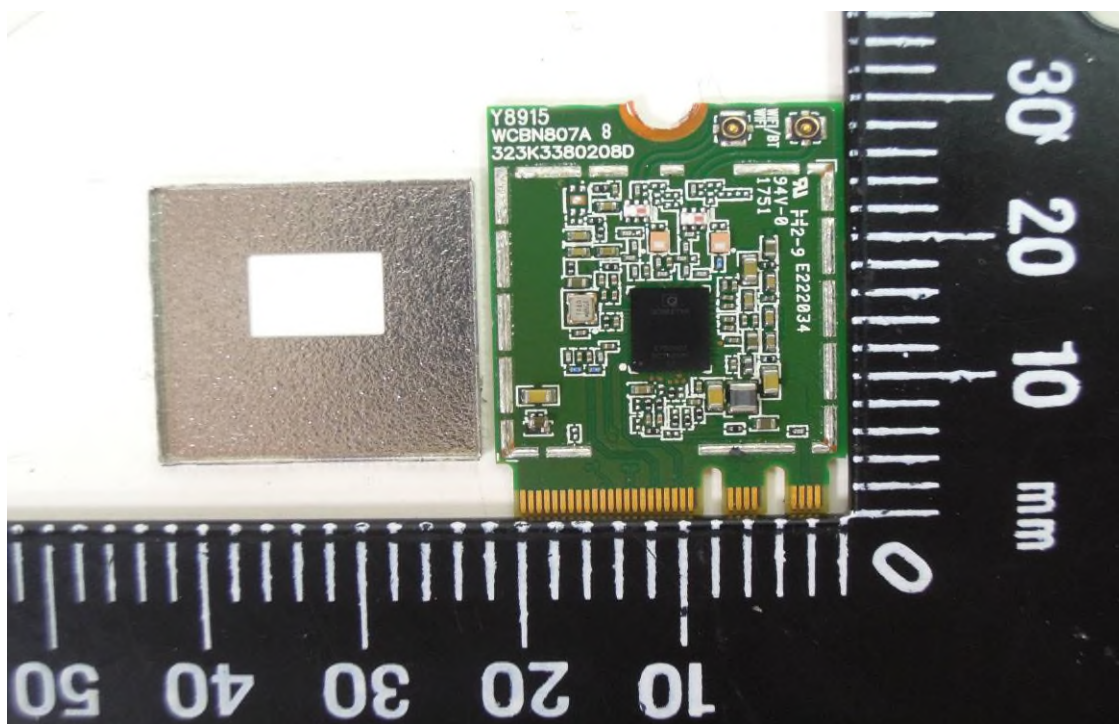
Internal View of EUT – 9
