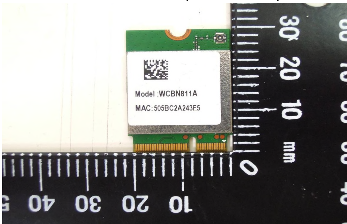
Internal View of EUT – 3 (Module Model: 811)
