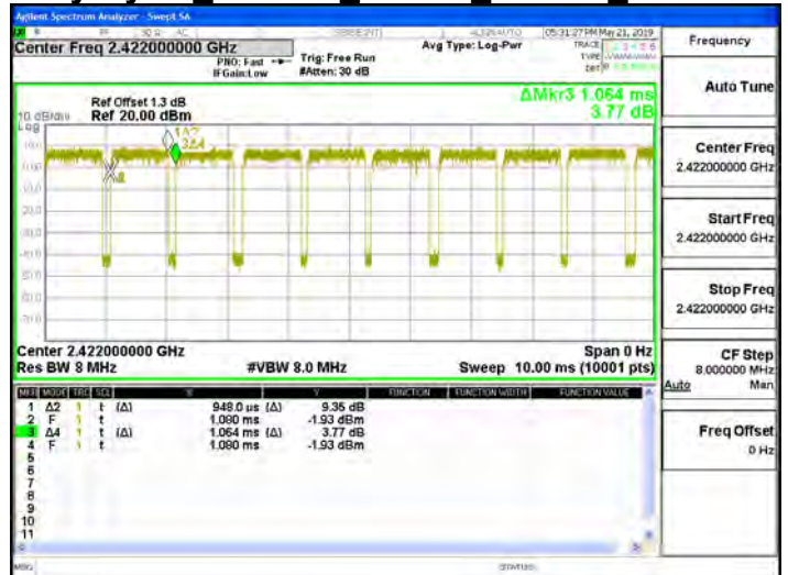
Duty Cycle 802.11n 40MHz Chain1 2422MHz
