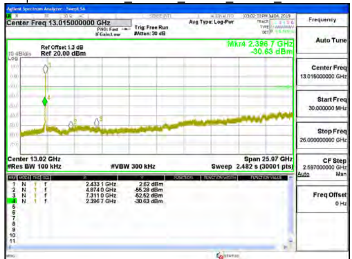
Spurious Emission 802.11n 40MHz Chain1 2452MHz
