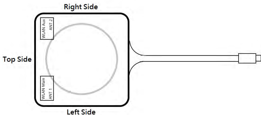
Fig.10 Antenna position of EUT
