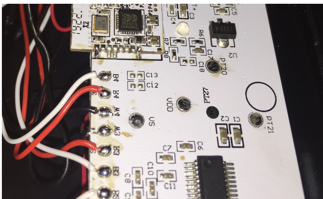
EUT – Chip View
