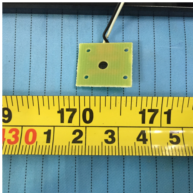
EUT – Keyboard Bottom View
