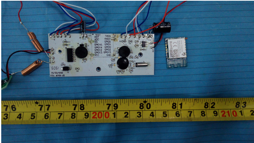
EUT – Cover off View 5
