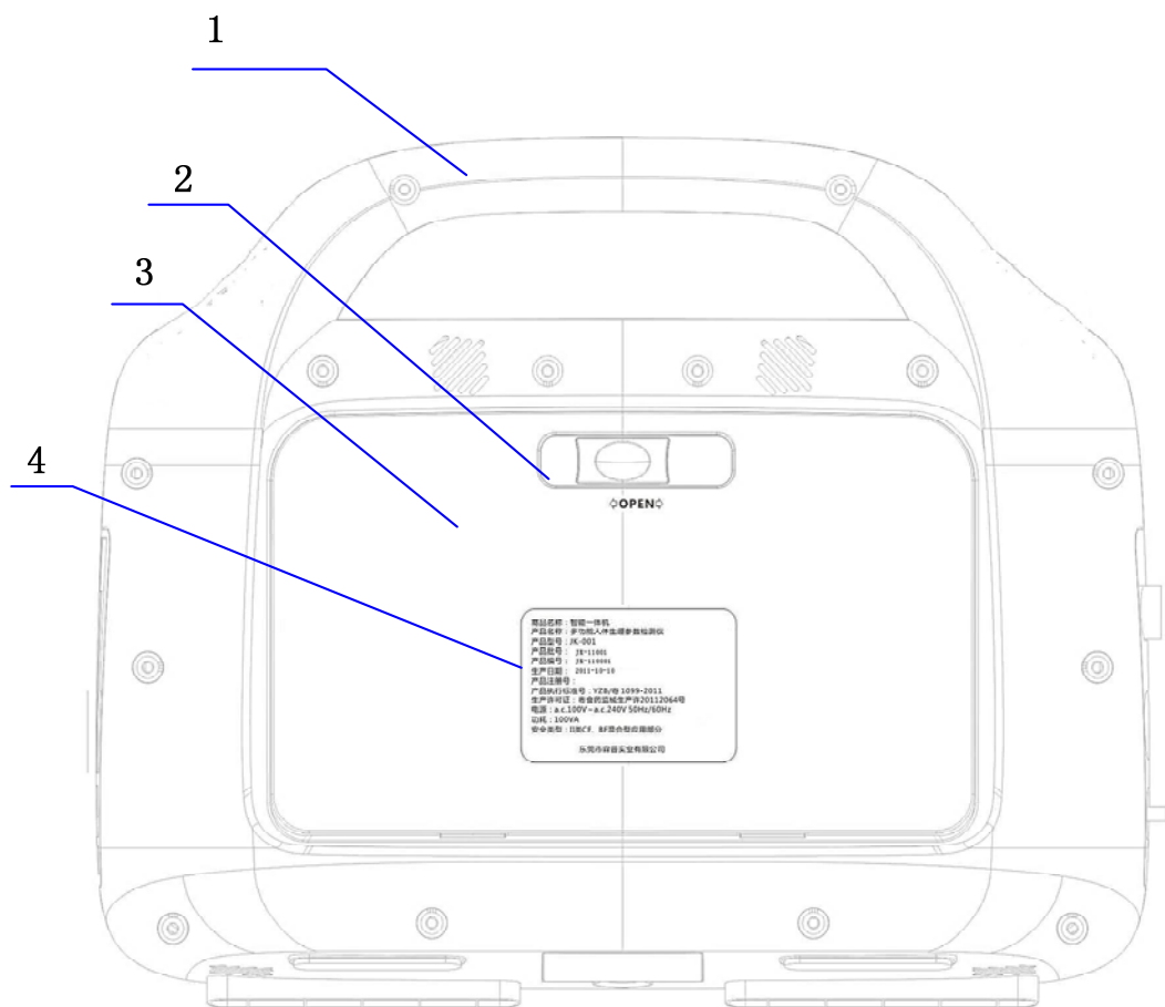
Figure 1-3 Rear-view
