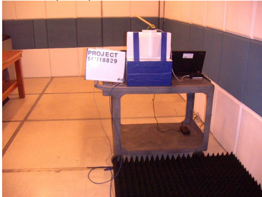
DFS SETUP (FRONT)
