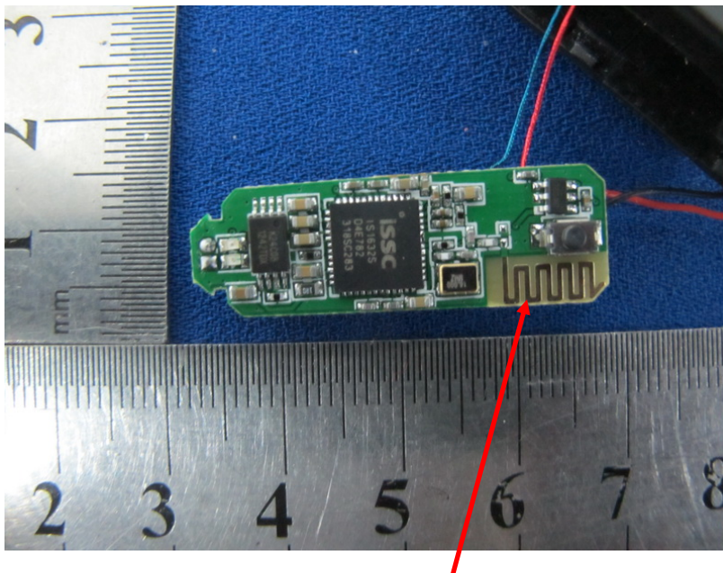
BT Antenna
