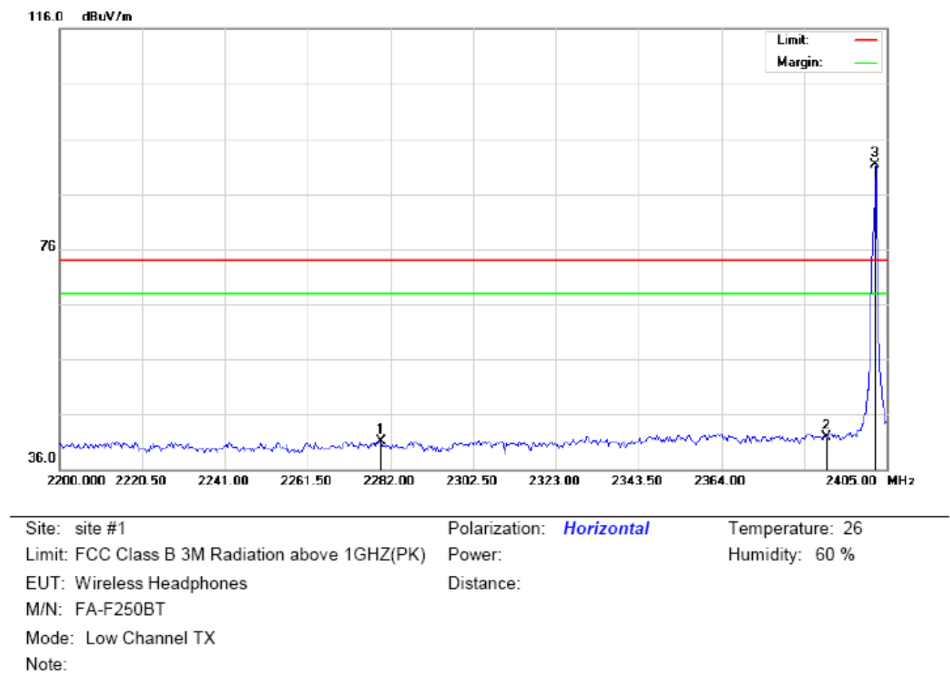
TEST PLOT OF BAND EDGE FOR LOW CHANNEL (1Mbps)-Horizontal
