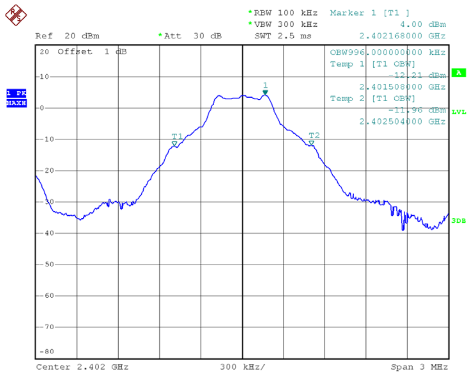
0 Channel @ GFSK
