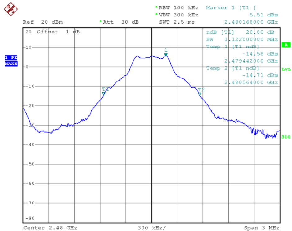
78 Channel @ GFSK
