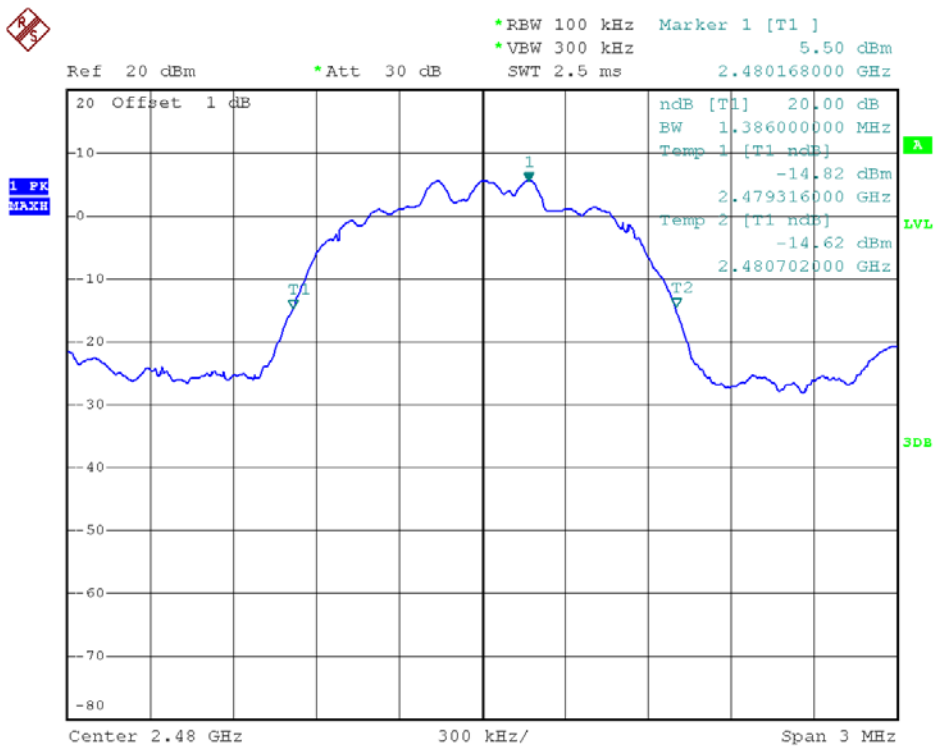
78 Channel @ 8-DPSK
