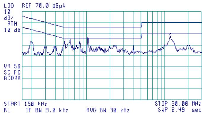
Plot 8.1.2 Conducted emission measurements
