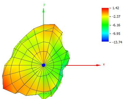
Theta = 0, Phi = 0
