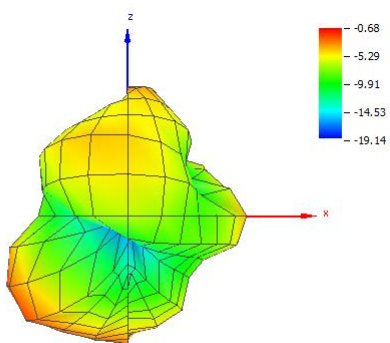
Theta = 90, Phi = 270
