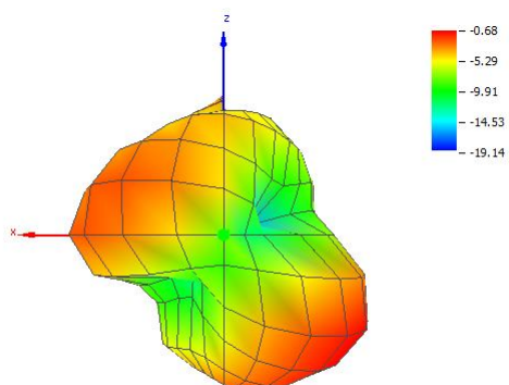
Theta = 90, Phi = 90
