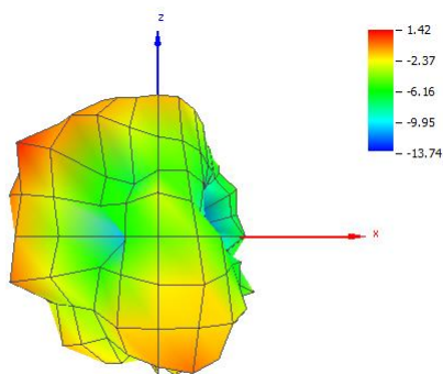
Theta = 90, Phi = 0
