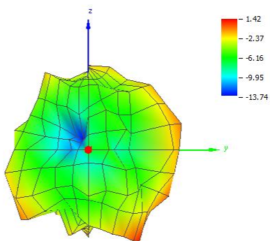
Theta = 0, Phi = 0
