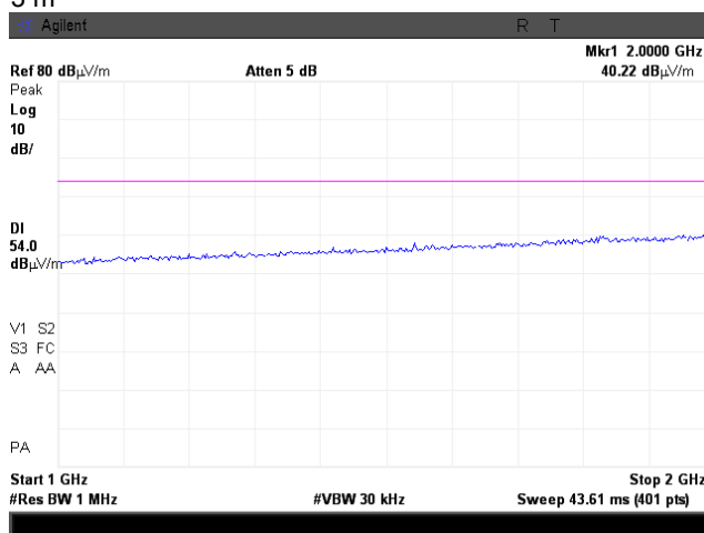
Plot 8.1.8 Radiated emission measurements above 1000 MHz, horizontal antenna polarization
