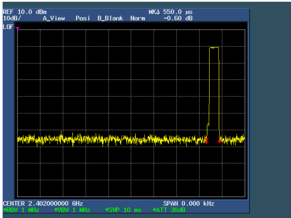
CH00-DH1
