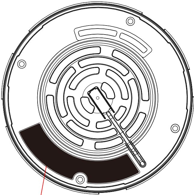
Product label(L) Size:53.4x26.2mm
