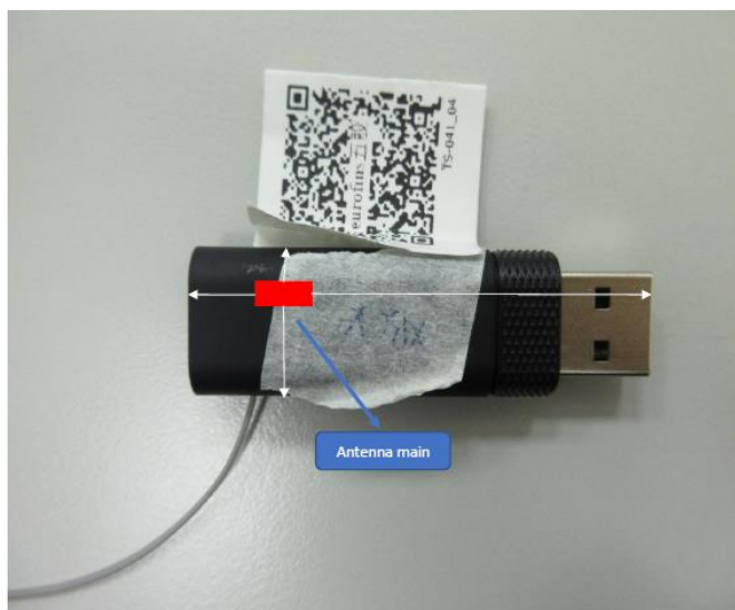
Dongle-Front View
