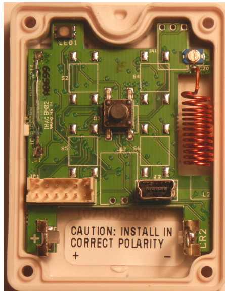
CT-101 - Front View
