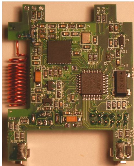
CT-101, CT-102, CT-104 - Rear View
