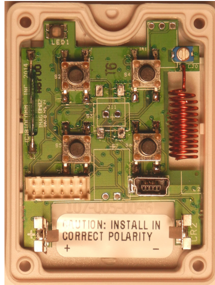
CT-102 & CT-104 - Front View
