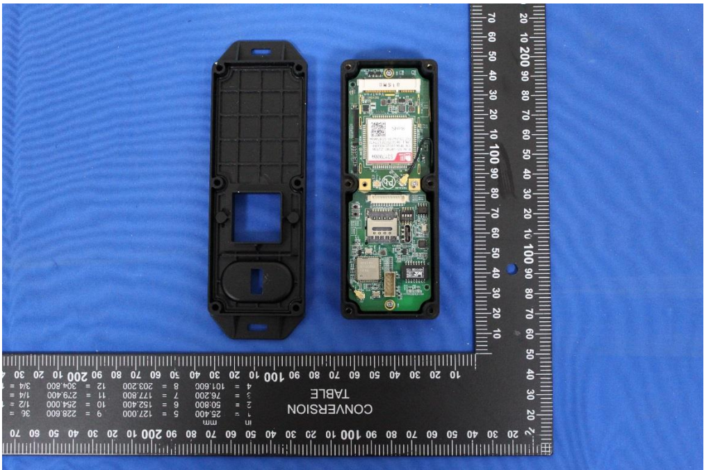
<VT-IoT-Dongle-CATM> Dismantling
