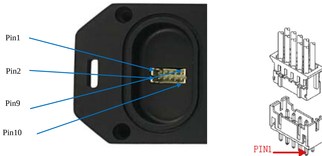
signal connector
