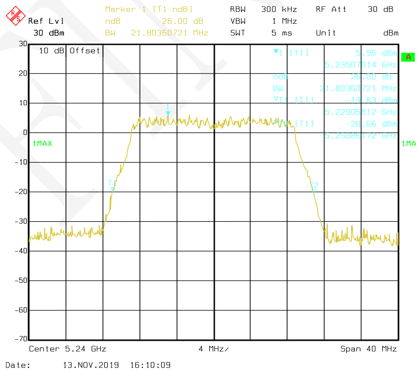
802.11ac20 mode, 26 dB Bandwidth-5240 MHz, Chain 1
