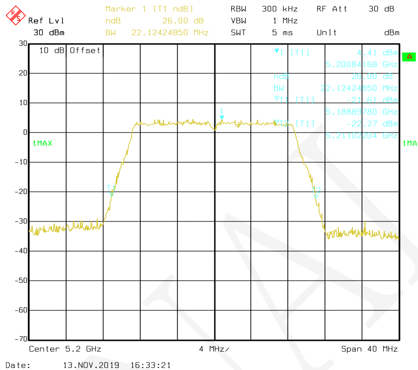
802.11ac20 mode, 26 dB Bandwidth-5200 MHz, Chain 1
