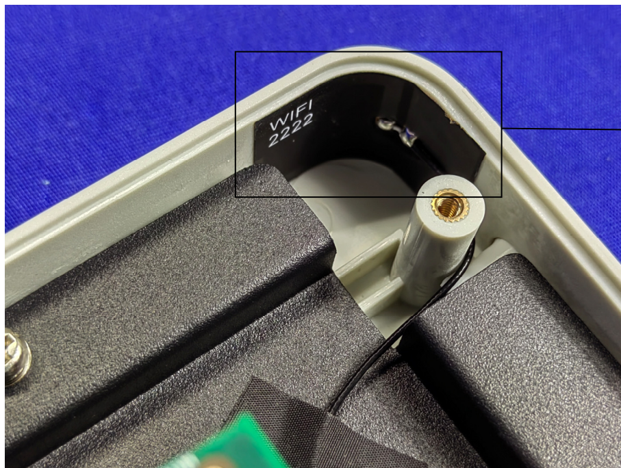
FPC Antenna
