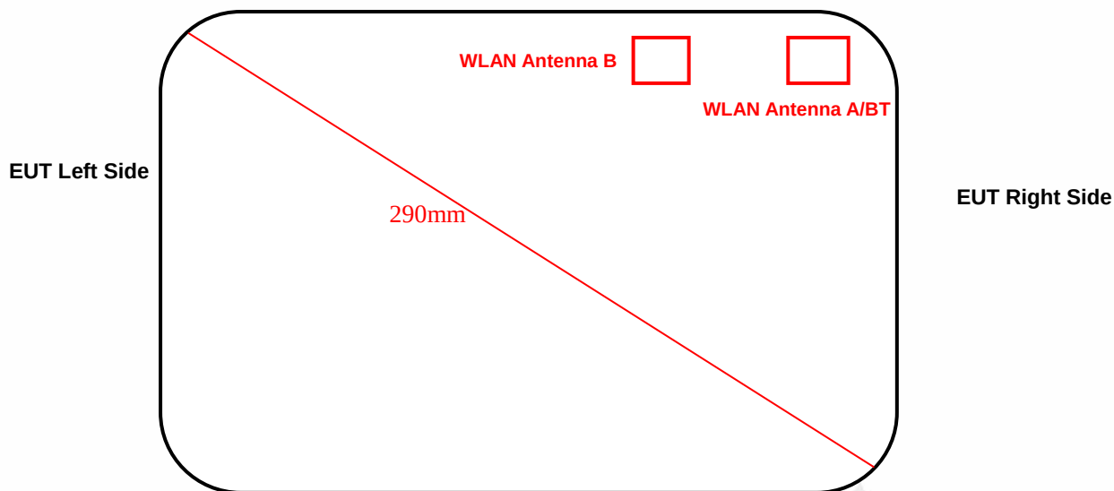
<EUT Front View>
