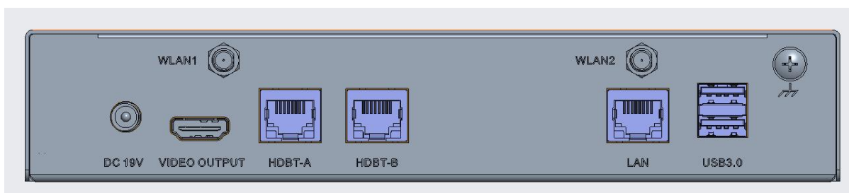
Figure 3-6 Part Bottom
