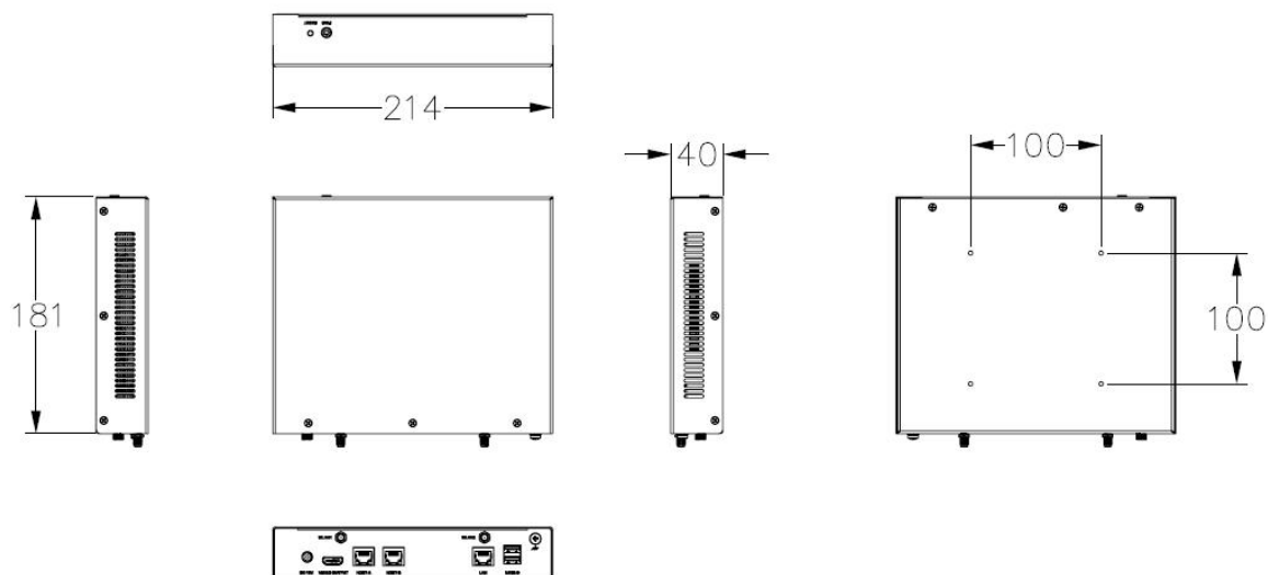
Figure 3-7 Dimensions
