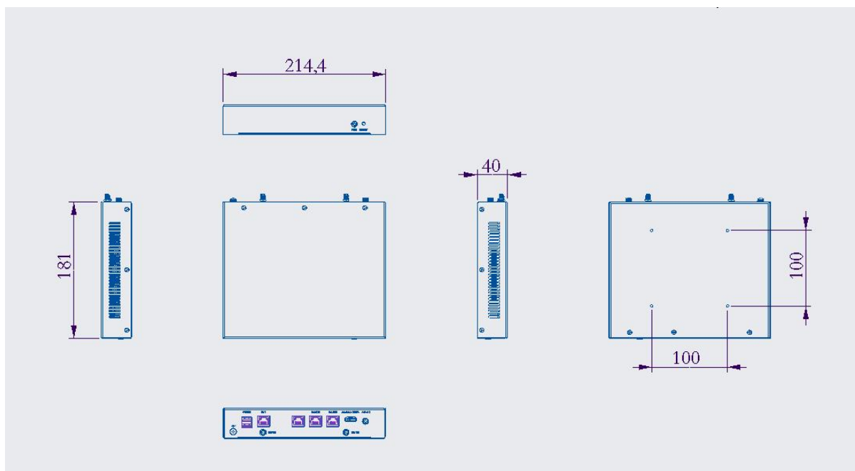
Figure 3-7 Dimensions
