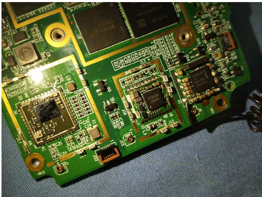
EUT – GPS Module Uncovered View
