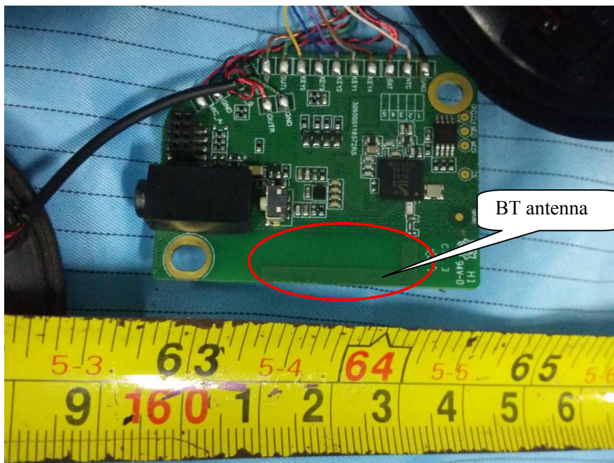
EUT – Mainboard 4 Front View
