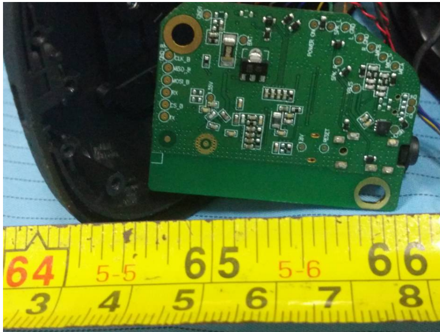
EUT – Mainboard 4 Rear View
