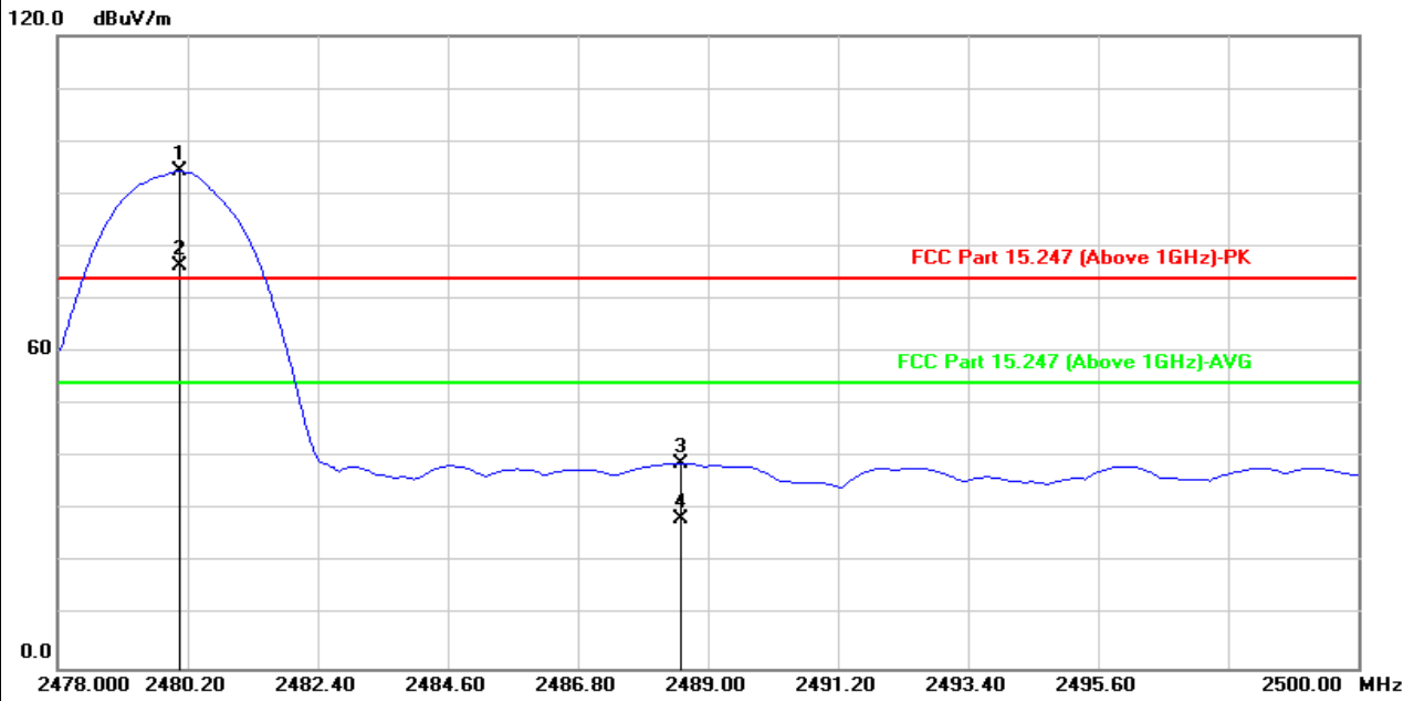
Antenna Polarity & Test Distance: Vertical at 3 m
