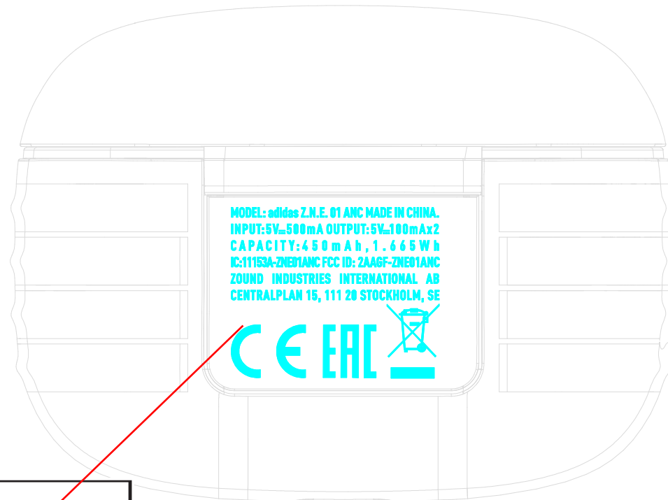
BACKSIDE CASE
