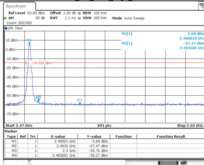
BLE_1M_Ant0_High_2480
