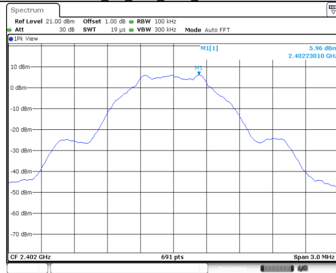
BLE_1M_Ant0_2402_0-Reference
