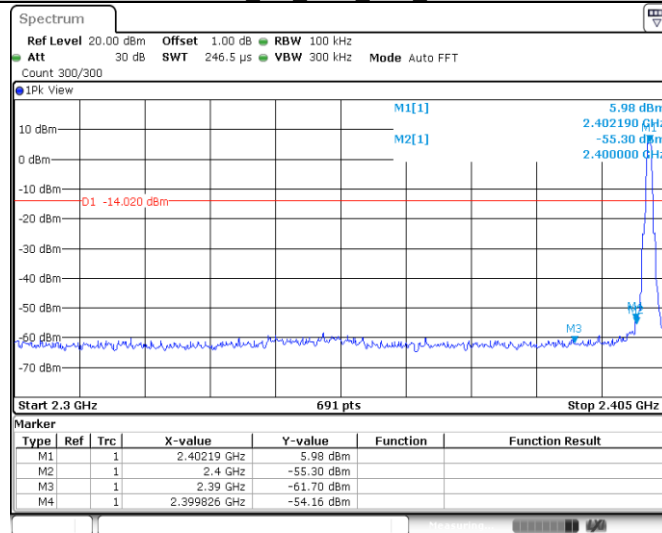
BLE_1M_Ant0_Low_2402
