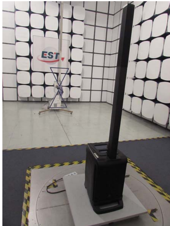
Radiated Test (30-1000 MHz)
