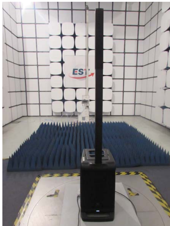
Radiated Test (1000-25000 MHz)
