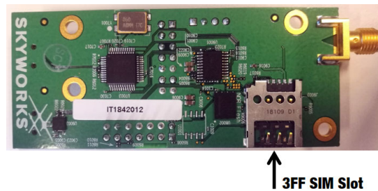
Figure 2. SKY66430-11 Evaluation Board Connector Diagram
