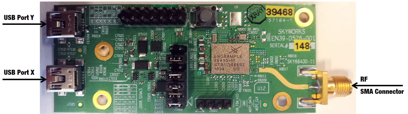
Figure 1. SKY66430-11 Evaluation Board Connector Diagram
