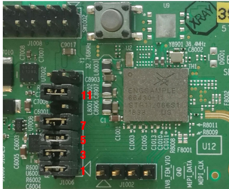
Figure 11. Default Jumper Settings
