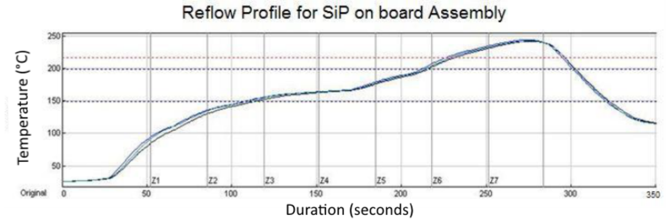
Figure 2-5: Reflow Profile
