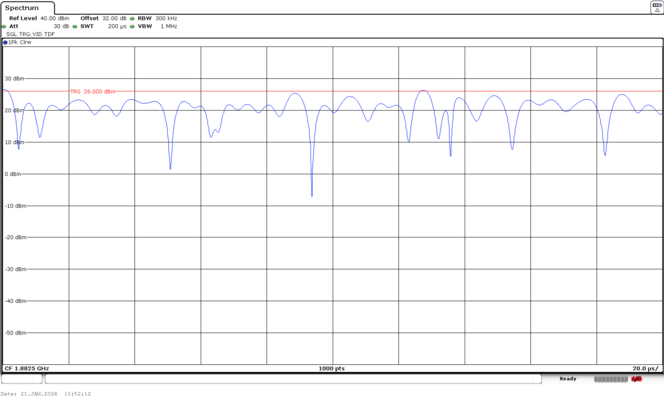
LTE Cat 1bis Band 2: BW=5 MHz. QPSK. RB Size=1. RB Offset=12. Middle Channel.
