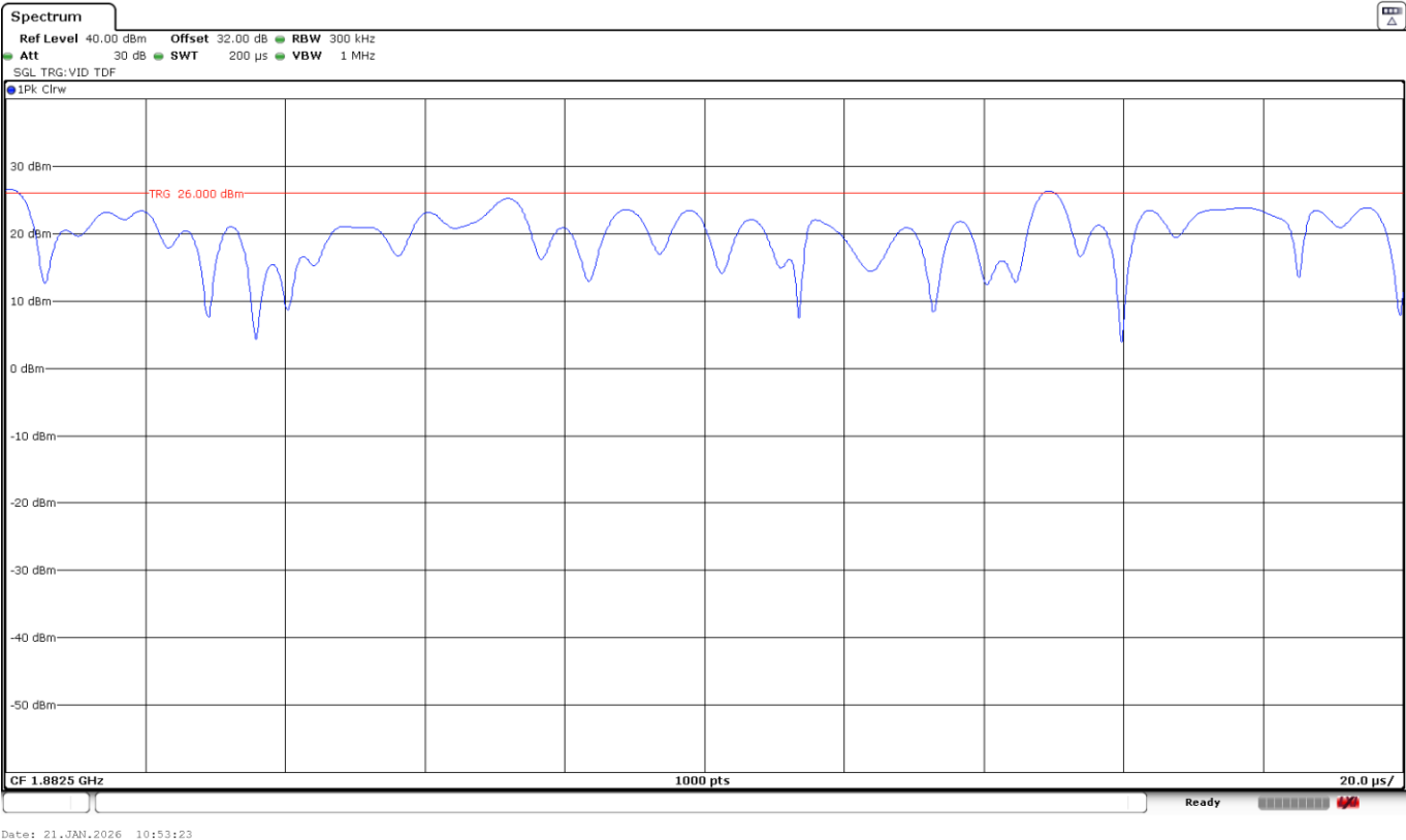
LTE Cat 1bis Band 2: BW=5 MHz. 16QAM. RB Size=1. RB Offset=12. Middle Channel.
