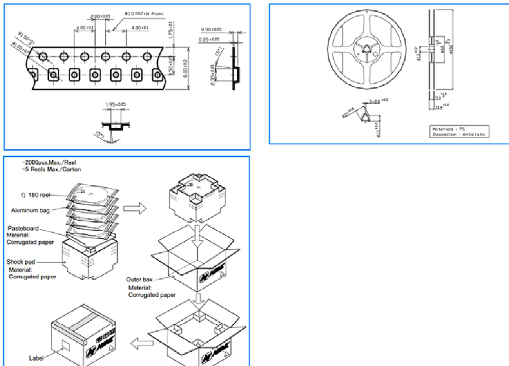
Figure 3-7: Packing Tape and Reel Description
