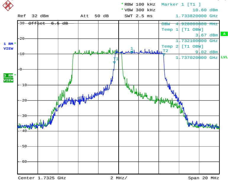
Figure 12: Band 4, BW=10MHz, 16-QAM (27 RB, Low and High)
