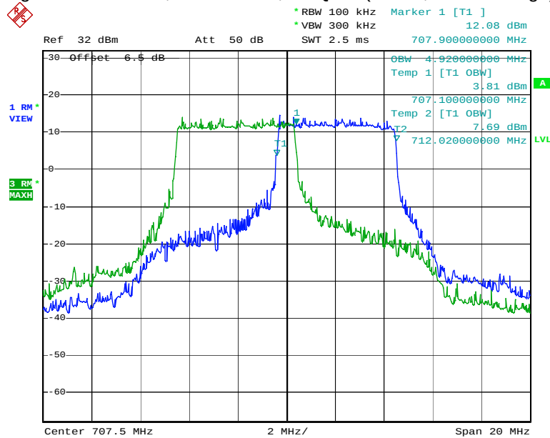
Figure 20: Band 12, BW=10MHz, 16-QAM (27 RB, Low and High)
