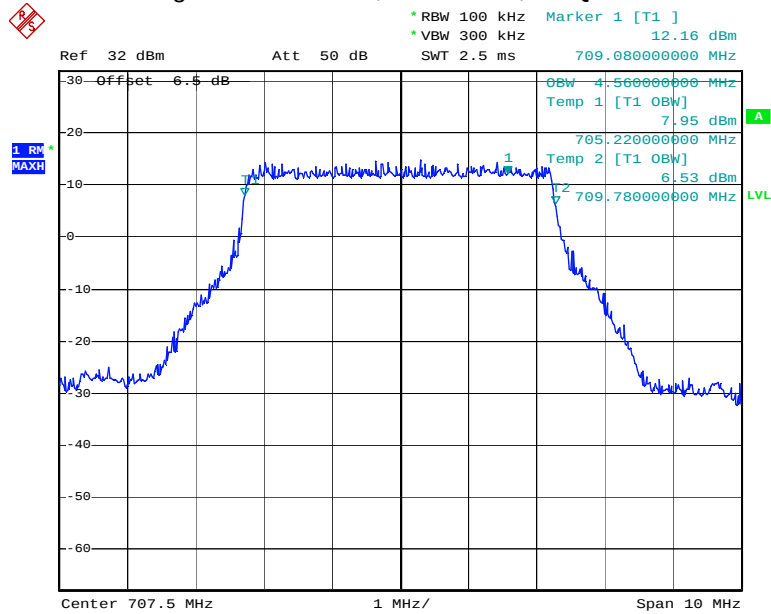
Figure 18: Band 12, BW=5MHz, 16-QAM
