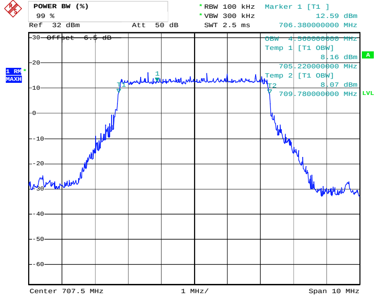
Figure 17: Band 12, BW=5MHz, QPSK
