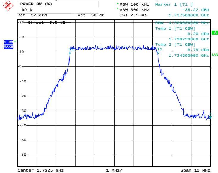
Figure 9: Band 4, BW=5MHz, QPSK
