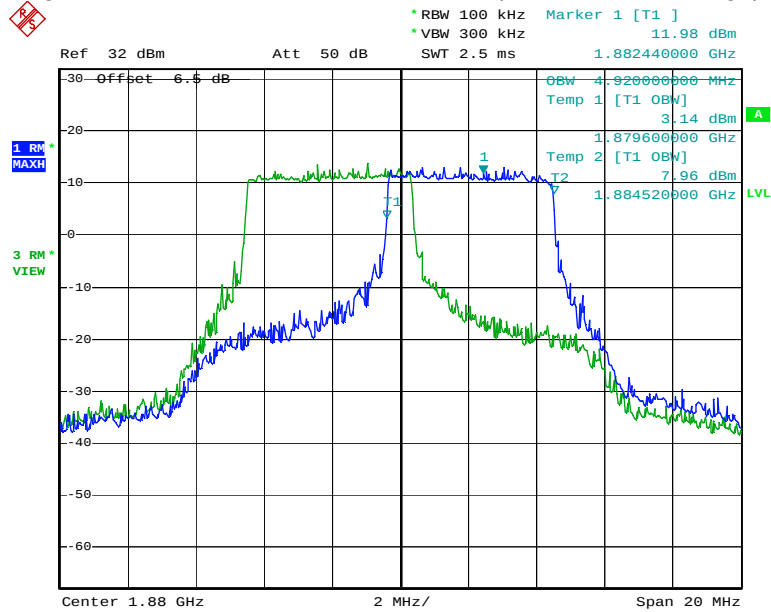
Figure 4: Band 2, BW=10MHz, 16-QAM (27 RB, Low and High)
