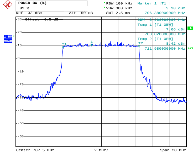
Figure 19: Band 12, BW=10MHz, QPSK
