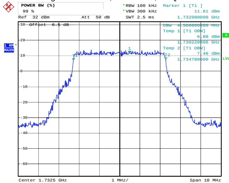
Figure 10: Band 4, BW=5MHz, 16-QAM
