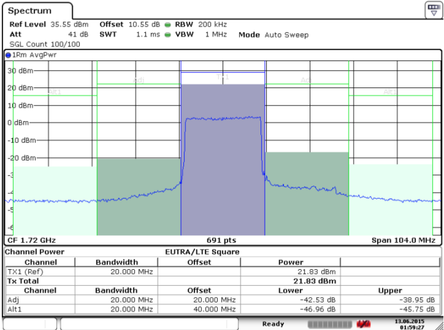
6.2.5.1.18 Figure 13 Avg Pwr Band4 lo_20
