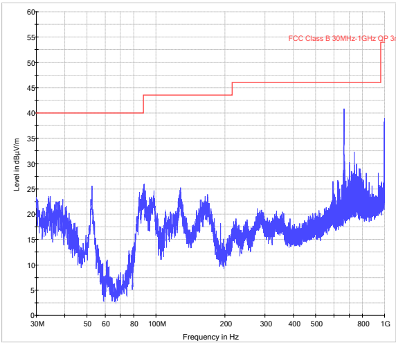
30MHz – 1GHz
