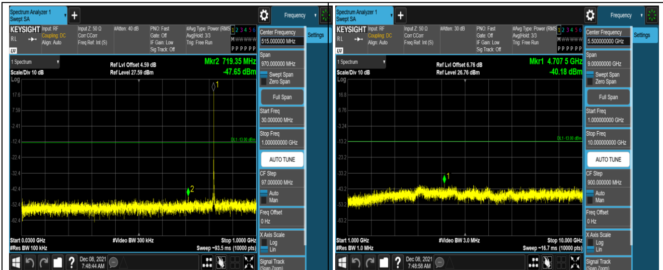
Band26-1.4MHz-16QAM-26797-1RB#0-Range1:30 ~1000MHz
