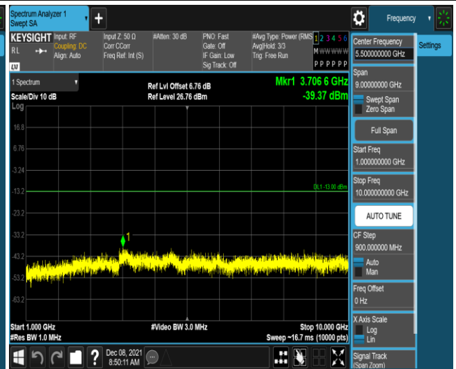
Band26-1.4MHz-16QAM-26740-1RB#0-Range2:1000 ~10000MHz
