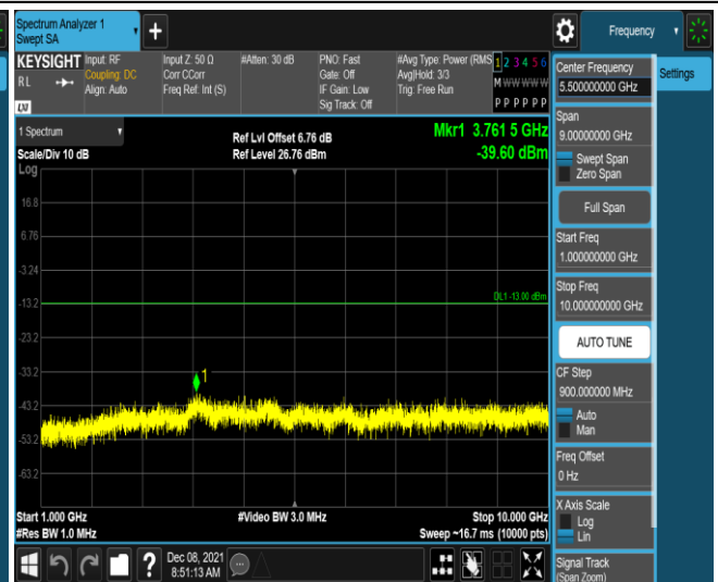
Band26-1.4MHz-16QAM-26783-1RB#0-Range2:1000 ~10000MHz
