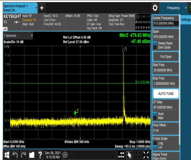
Band26-10MHz-QPSK-26740-1RB#0-Range1:30~1 000MHz
