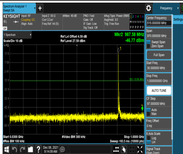
Band26-10MHz-16QAM-26740-1RB#0-Range1:30~ 1000MHz
