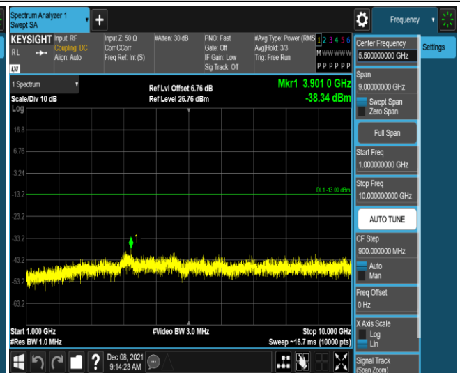
Band26-10MHz-16QAM-26740-1RB#0-Range2:1000 ~10000MHz
