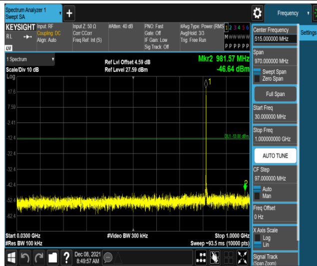
Band26-1.4MHz-16QAM-26740-1RB#0-Range1:30 ~1000MHz
