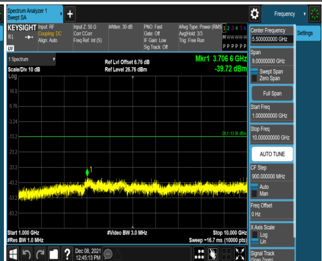
Band71-20MHz-16QAM-133222-1RB#0-Range2:1000~10000MHz
