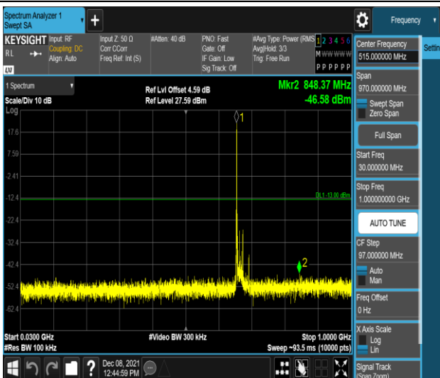
Band71-20MHz-16QAM-133222-1RB#0-Range1:30~1000MHz
