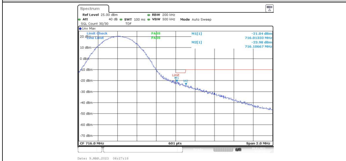
Band17-10MHz-16QAM-23800-50RB#0
