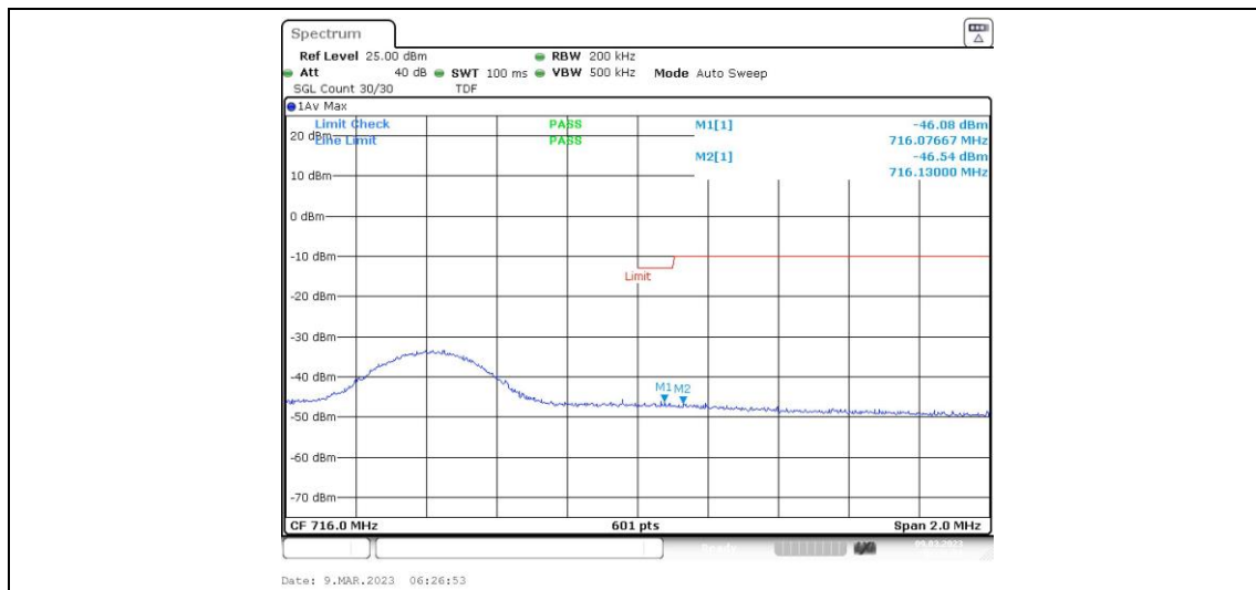
Band17-10MHz-16QAM-23800-1RB#49
