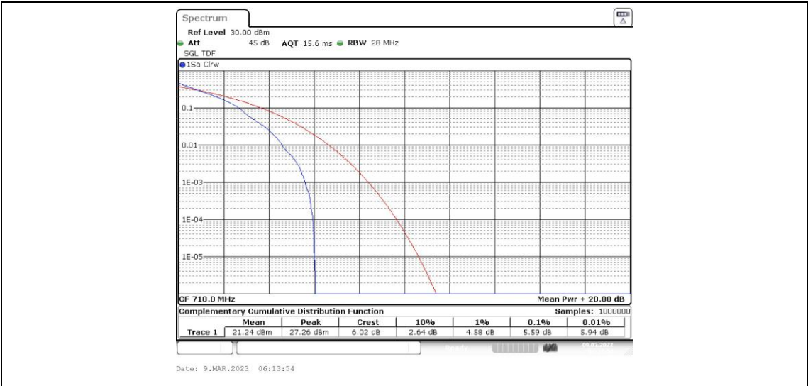
Band17-5MHz-QPSK-23790-25RB#0
