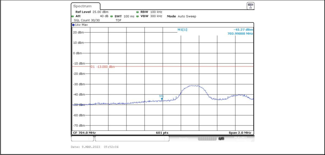
Band17-5MHz-QPSK-23755-25RB#0
