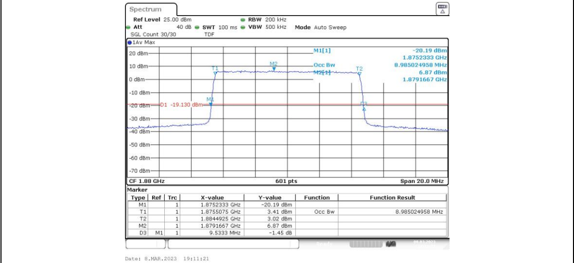
Band2-10MHz-QPSK-19150-50RB#0
