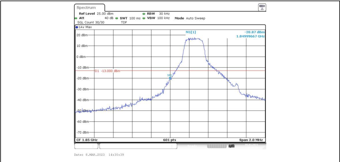
Band2-1.4MHz-QPSK-18607-1RB#5
