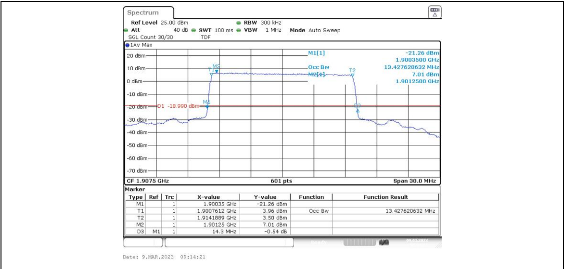
Band25-15MHz-16QAM-26115-75RB#0
