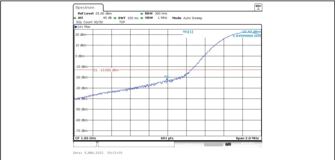
Band25-15MHz-QPSK-26115-1RB#74
