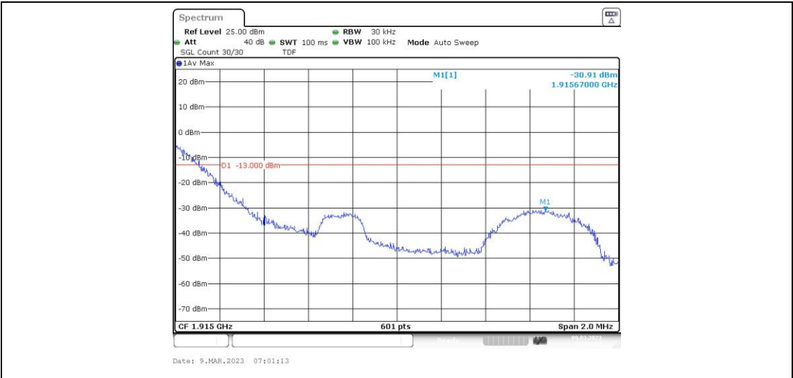
Band25-1.4MHz-QPSK-26683-1RB#5
