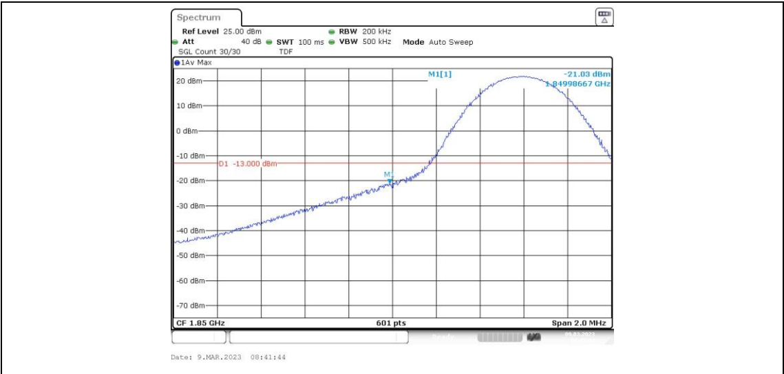
Band25-10MHz-QPSK-26090-1RB#49
