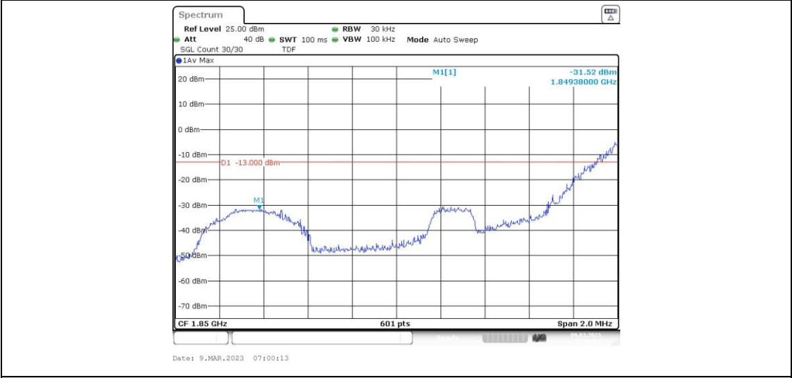
Band25-1.4MHz-QPSK-26047-6RB#0
