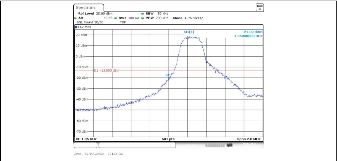
Band25-3MHz-16QAM-26055-1RB#14
