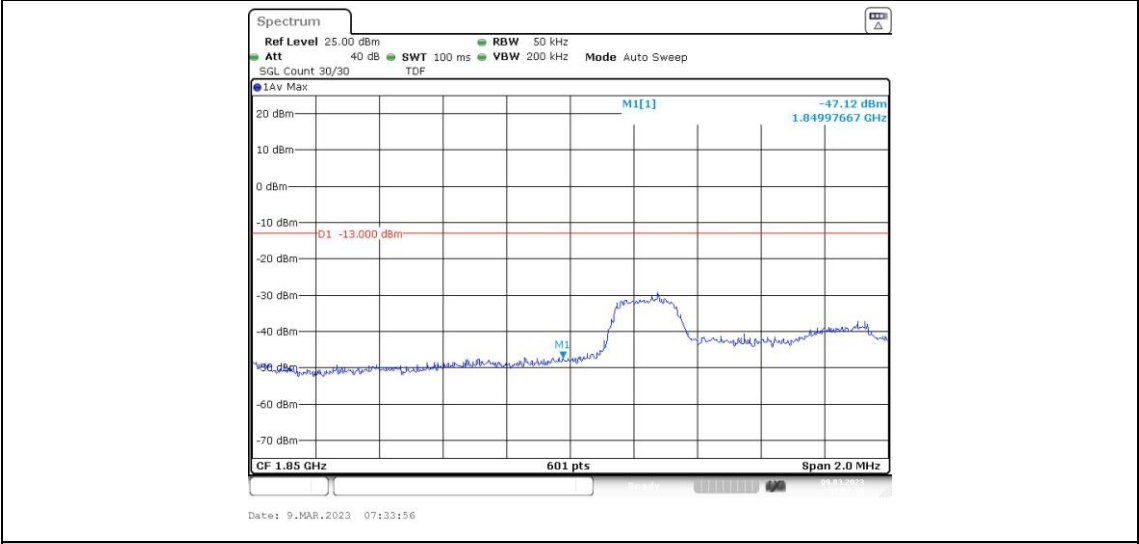
Band25-3MHz-16QAM-26055-15RB#0
