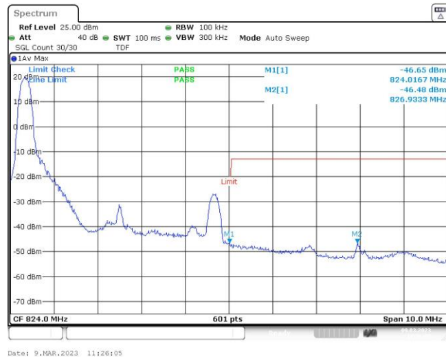
Band26-5MHz-16QAM-26765-1RB#24
