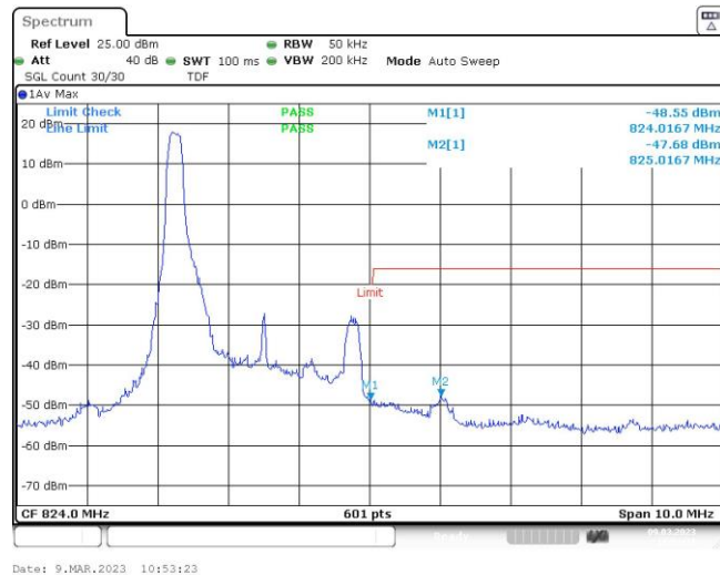
Band26-3MHz-16QAM-26775-1RB#14
