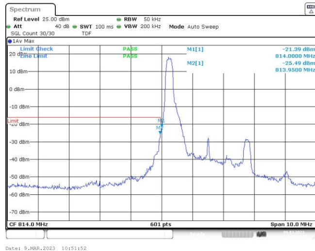
Band26-3MHz-16QAM-26705-1RB#14
