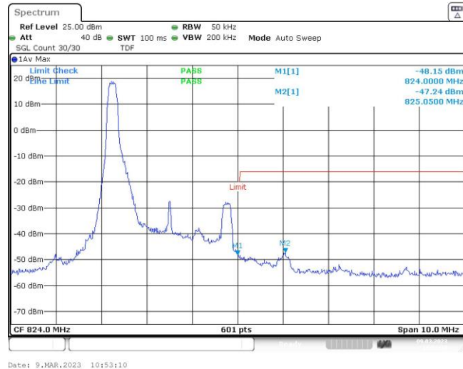
Band26-3MHz-QPSK-26775-1RB#14
