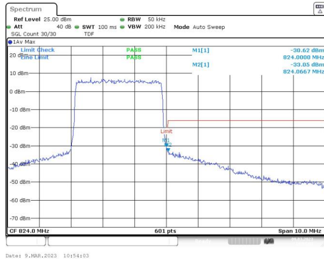
Band26-3MHz-16QAM-26705-1RB#0
