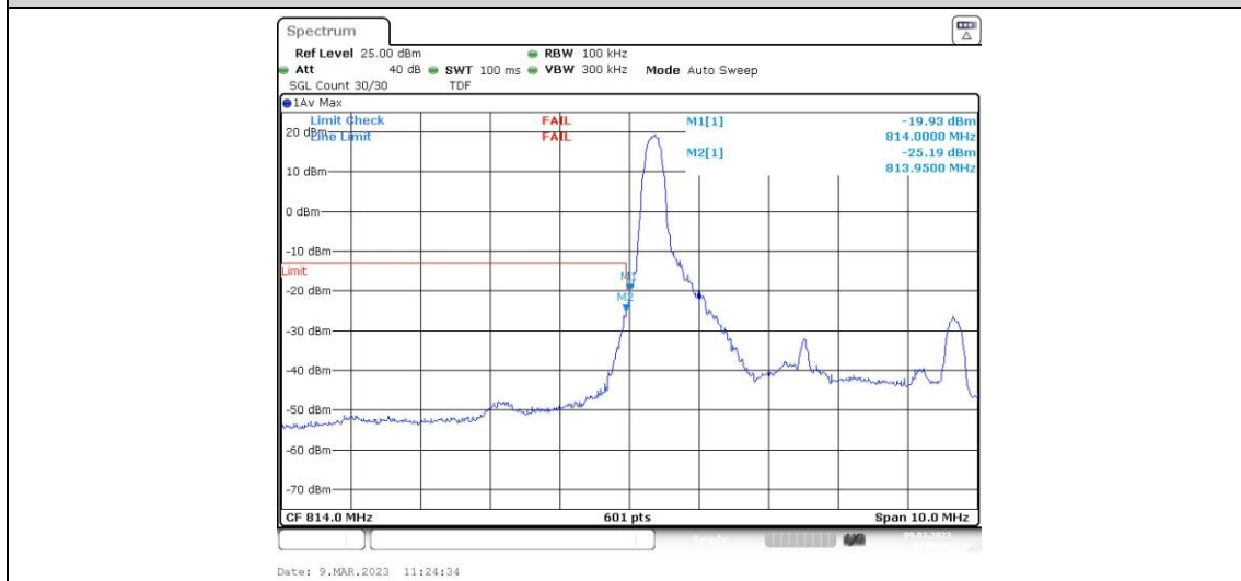
Band26-5MHz-16QAM-26715-1RB#24
