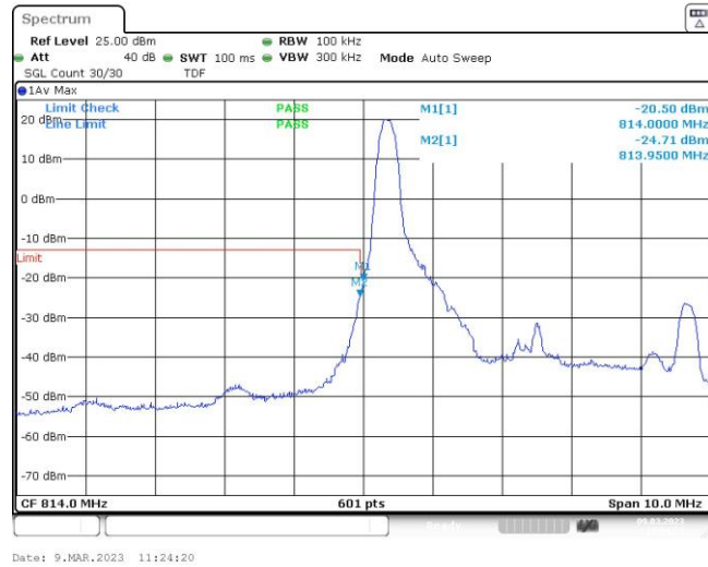
Band26-5MHz-QPSK-26715-1RB#24
