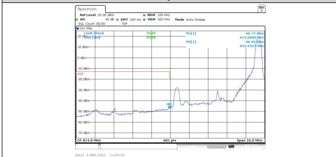
Band26-5MHz-16QAM-26715-25RB#0
