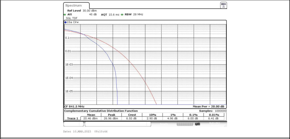
Band26-15MHz-16QAM-26965-75RB#0
