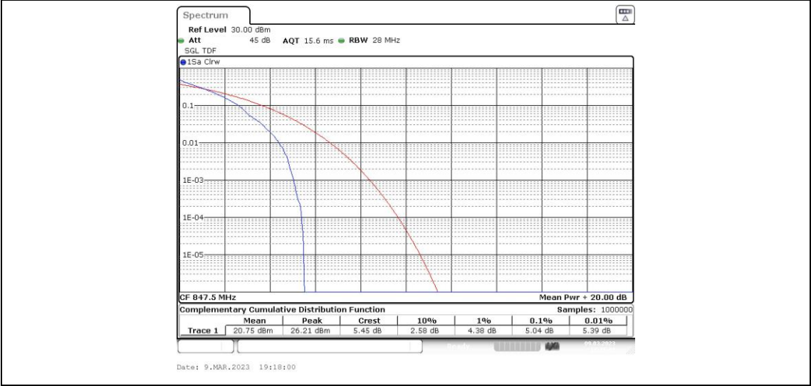
Band26-3MHz-QPSK-27025-15RB#0
