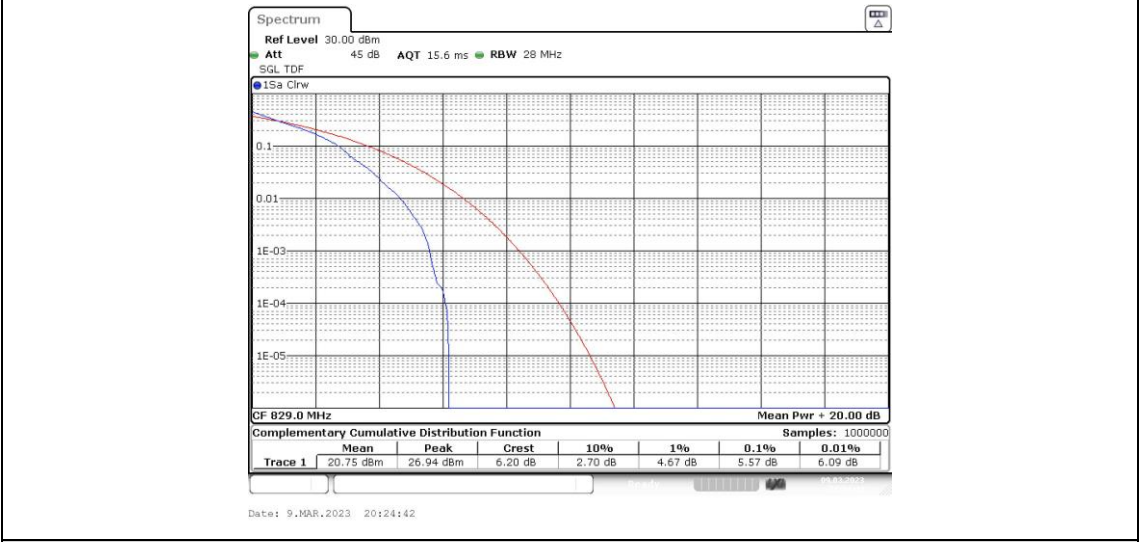
Band26-10MHz-QPSK-26840-50RB#0
