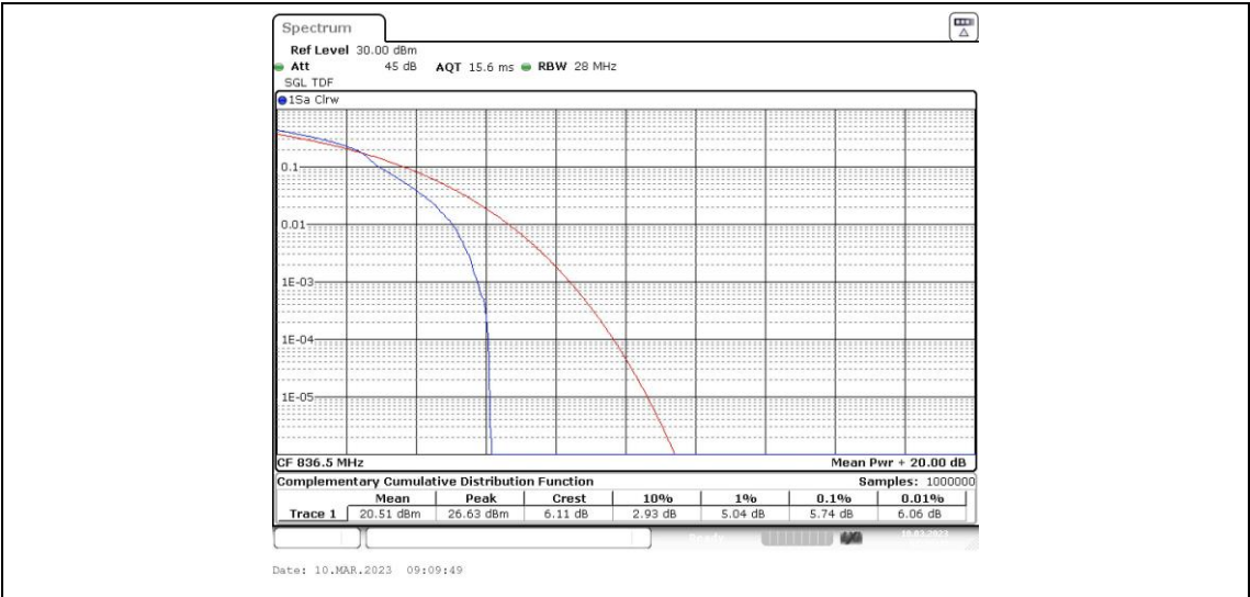
Band26-15MHz-16QAM-26915-75RB#0
